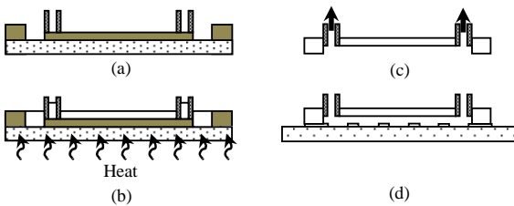
Fig. 7 Fabrication process of the microfluidic device
