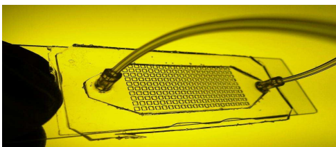
Fig. 8 The complete microfluidic device
