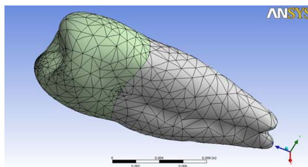
Fig. 4 Finite element model of the maxillary first premolar
