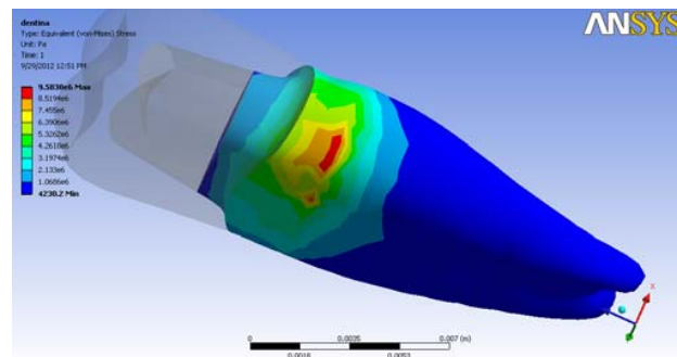
Fig. 7 Stress distribution in the prepared tooth
