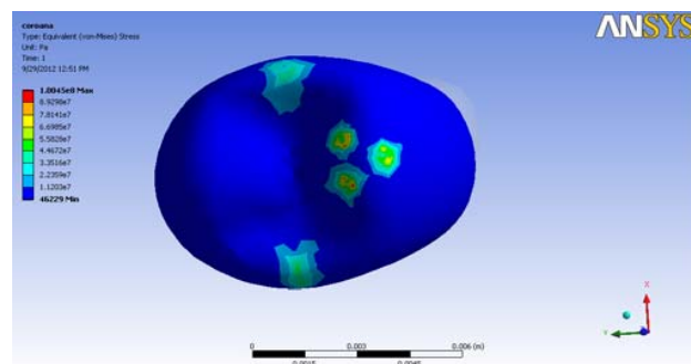
Fig. 8 Stress distribution in the overlying crown
