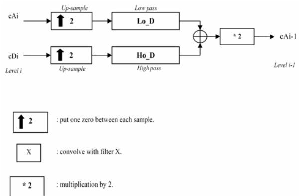
Fig. 3 The algorithm of the IDWT
