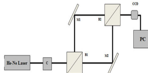
Fig. 1 Schematics of Mach-Zehnder interferometer
