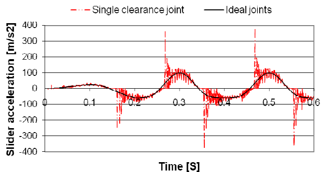
Fig. 8 Slider acceleration at at \omega = 300 rpm
