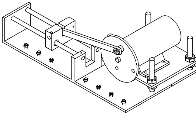
Fig. 13 Mechanism construction: slider – crank mechanism (isometric)
