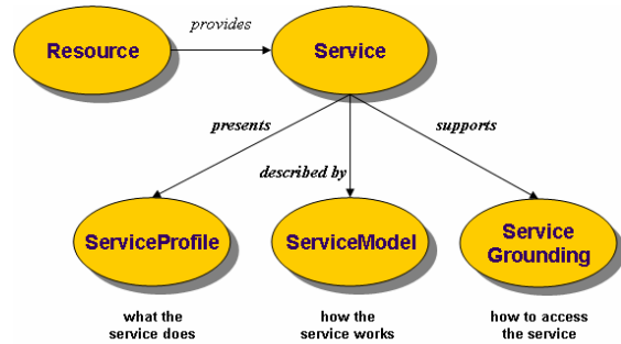
Fig. 4 Organization of OWL-S into modules
