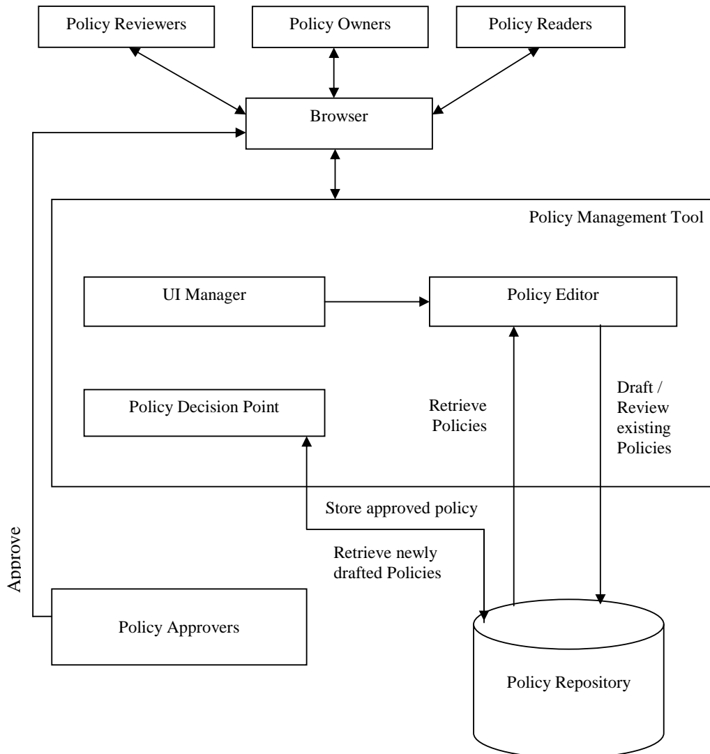
Fig. 2 Proposed Policy management framework
