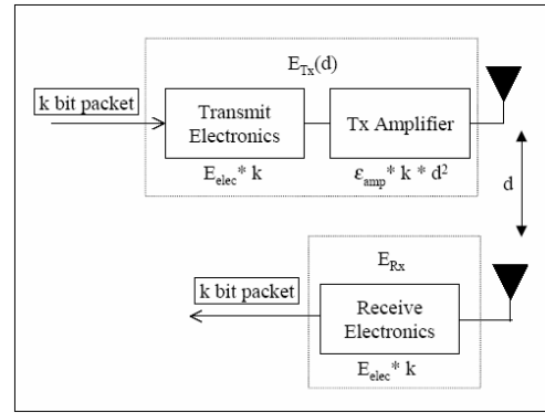
Fig. 1 First order radio model
