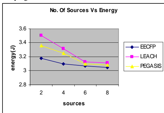
Fig. 7 Sources Vs Energy
