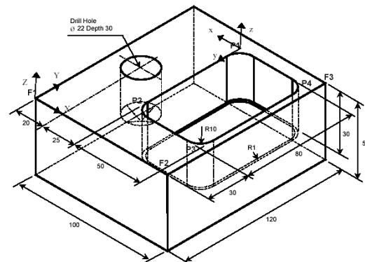
Fig. 4 Example of workpiece
