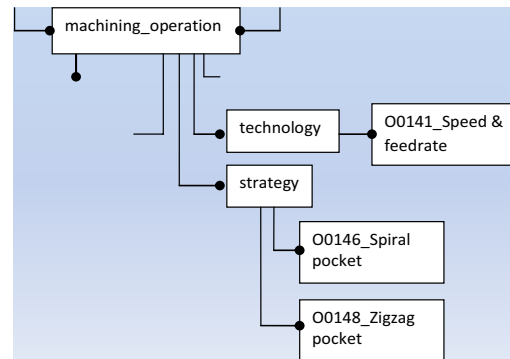
Fig. 3 Example of how macros are implemented
