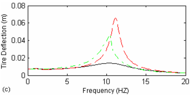
Fig. 3 Frequency analysis of 4DOF model a) Body acceleration b) Roll angle c) Tire deflection
