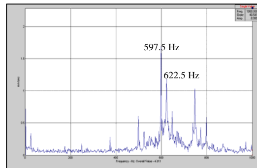
Fig. 4 Frequency spectrum of the pump drive end bearing
