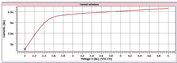
Fig. 6. Output current under varying supply voltage.
