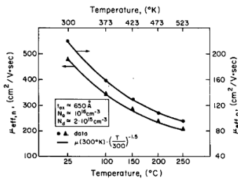
Fig. 2. Effective channel mobility versus temperature characteristics for n and p channel MOSFET. [2]
