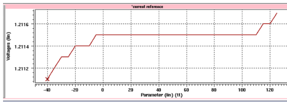
Fig. 9. Output voltage at varying temperature.
