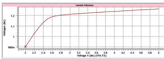
Fig. 10. Output voltage under varying supply voltage.
