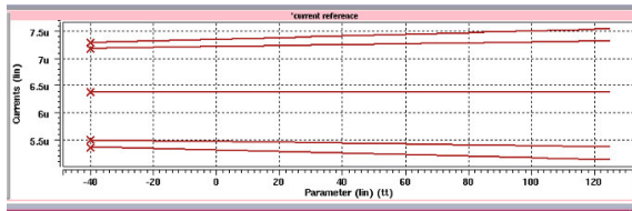
Fig. 8. Current reference under the five corner condition.
