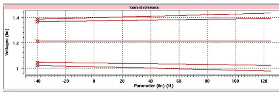
Fig. 12. Current reference under the five corner condition.
