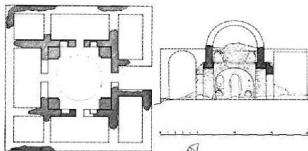
Fig.13 Plan and the cross-section of cross-vault “Kerateh” (northwest of “Duzeh” in Fars)
