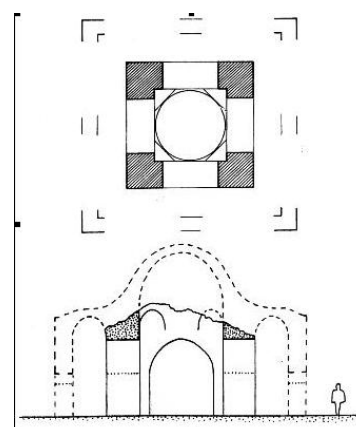
Fig.22 Exploration around Nevis-Tafrish cross-vault and the evidence to circumferential wall which made a narrow hall around square shape dome-house
