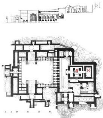
Fig.3 Plan and vertical section of the fire-temple in the mountain
