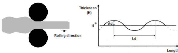
Fig. 4 Entry strip thickness deviation
