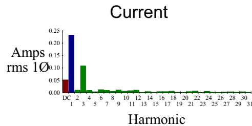
Fig. 9 Measured input supply current spectrum
