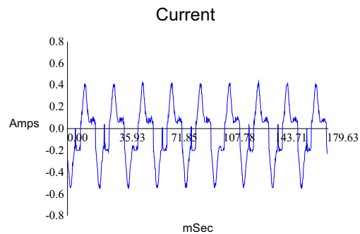
Fig. 8 Measured input supply current waveform
