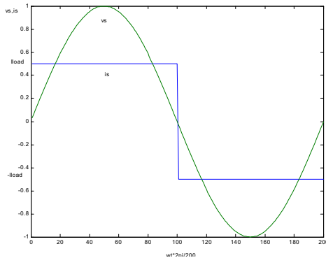
Fig. 3 The voltage & current of an idealized diode rectifier
