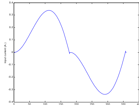
Fig. 7 Simulated input supply current
