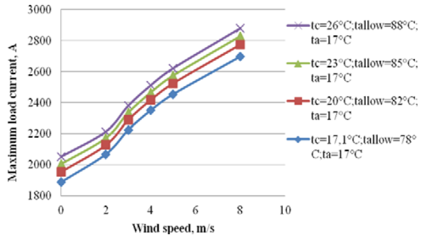
Fig. 7 Maximum load current for the second variant of examined conditions
