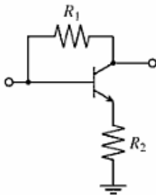
Fig.2, Negative resistive feedback circuits [1]
