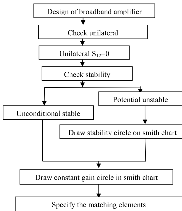
Fig.8, Block diagram of proposed approach
