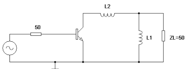
Fig.7, schematics diagram of a broadband amplifier
