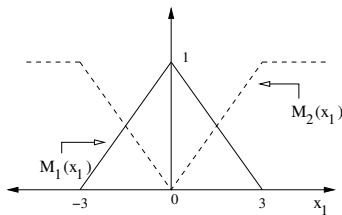
Fig. 2. Membership functions for the two fuzzy set.
