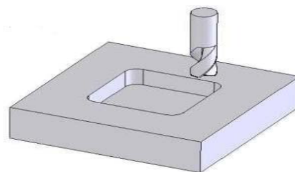
Fig. 2 A simple pocket milling operation
