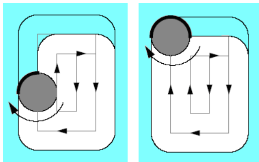
Fig. 3 Varying radial tool engagement in pocket milling
