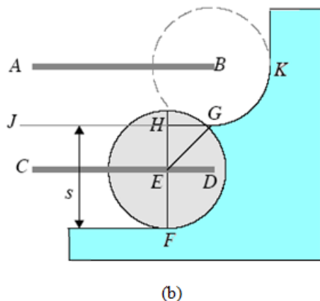
Fig. 5 Material being cut from left to right [14]
