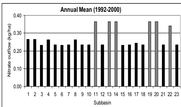
Fig. 6 Simulated annual average of per-unit-area \text{NO}_3\text{-N} outflow from each subbasin under existing land use/cover condition
