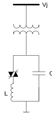
Fig. 2. Basic SVC topology
