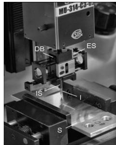
Fig. 1 Picture of indenter-specimen interaction: (DB) device body, (ES) elastic strips, (I) indenter, (IS) indenter support, (S) specimen
