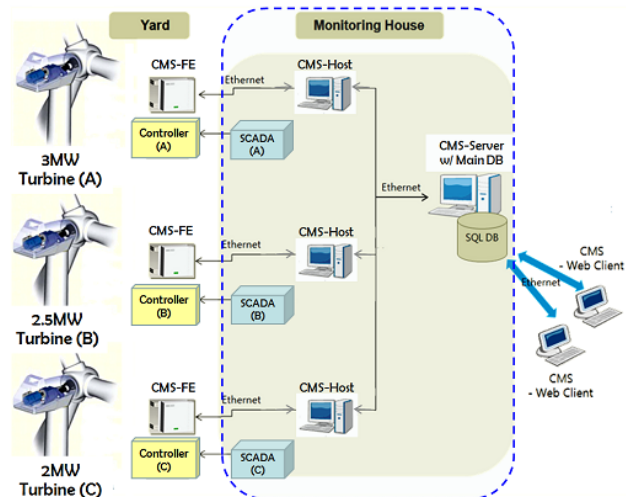
Fig. 5. Original overall structure for YeungHeung wind test bed.
