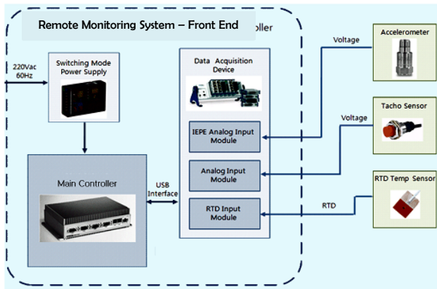
Fig. 7 Structure of CMS-FE
