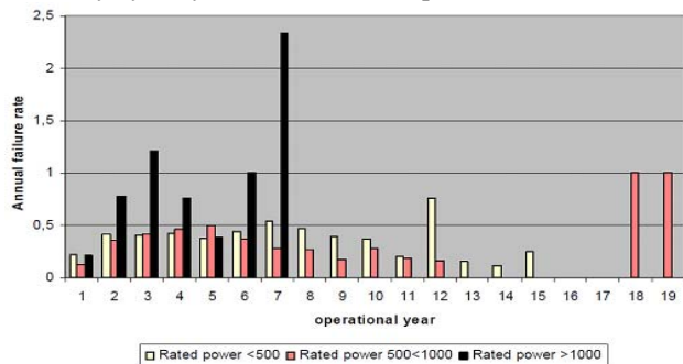
Fig. 2 Annual failure rate according to operational year[2]
