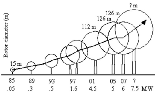
Fig. 1 Wind turbine size evolution[1]
