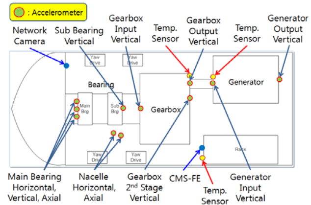
Fig. 8 Installation example of sensors and camera.
