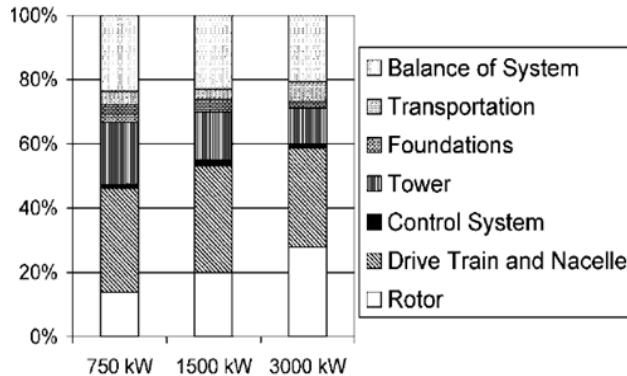
Fig. 3 Cost of wind turbine components[5]
