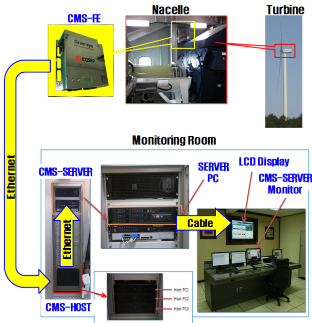
Fig. 11. Developed condition monitoring system
