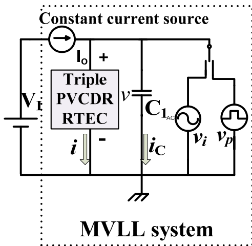
Fig.8 Improved critical four levels MVLL system using basic triple PVCDCR RTEC
