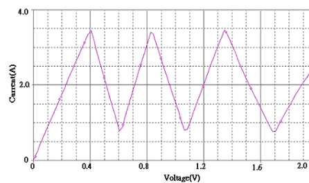
Fig.4 I-V characteristic of triple PVCDR RTEC element with three NDR curves
