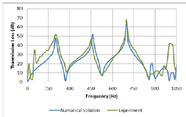
Fig. 7 Transmission loss
