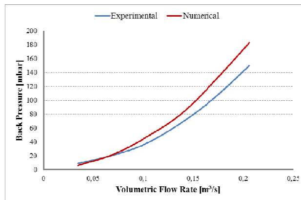
Fig. 9 Back pressure values vs. volumetric flow rate
