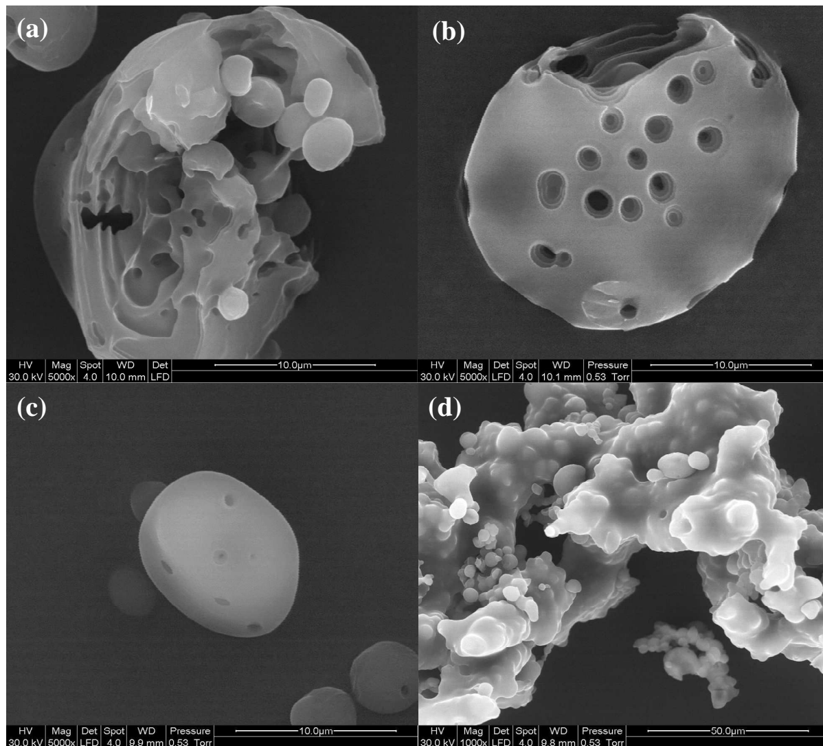
Fig. 4 ESEM images post digestion at magnification 5000×(a) = original wheat starch, (b) = granules >10\mu\text{m} , (c) = granules <10\mu\text{m} , (d) = granules <10\mu\text{m} at magnification 1000×
