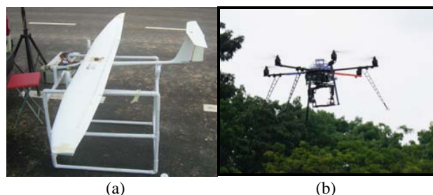
Fig. 1 (a) Fixed wing UAV; (b) Multi-rotor UAV
