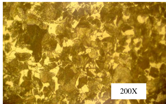
Fig. 9 Microstructure of annealed specimen
