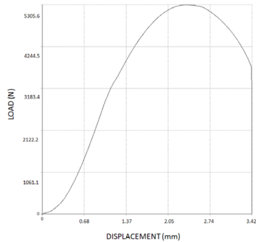
Fig. 13 Load-Displacement Diagram
