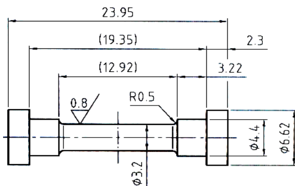
Fig. 3 Tensile Test Specimen
