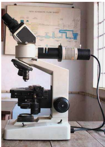
Fig. 7 Metallurgical Microscope
