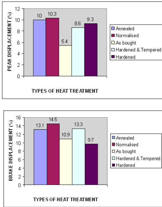
Fig. 15 Variation in ductility values w.r.t. different treatments
