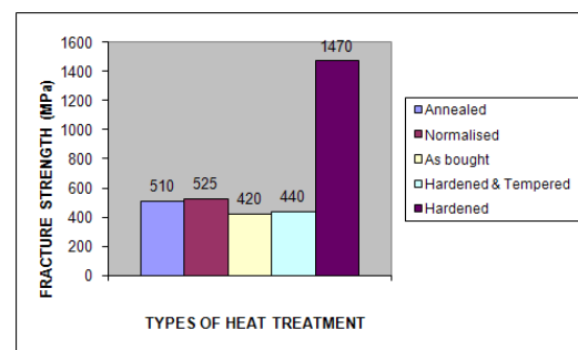
Fig. 14 Variation in strength values w.r.t. different treatments
