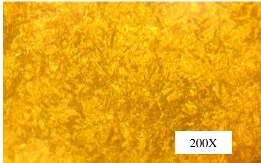
Fig. 11 Microstructure of hardened specimen
