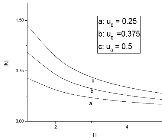
Fig. 2 Variation of |k_i| (for one typical mode) with quantum parameter H for different values of the streaming velocity u_0 (0.25, 0.375 and 0.5), where, d=5 , p_{01}=2.4048 , \sigma=0.01 , \delta=0.1 , \omega=0.1 and \mu=0.5
