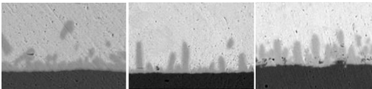
Fig. 2 SEM Backscattered electron micrographs illustrating the solder SAC-Ce-Fe on Cu substrate after reflow at (a) 220°C (b) 230°C and (c) 240°C respectively
