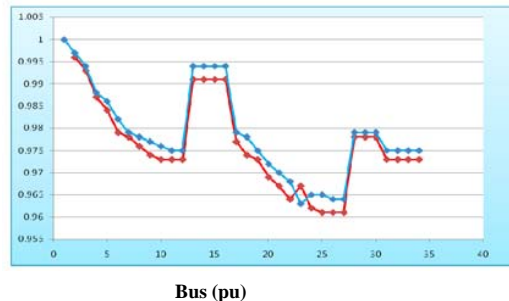
Fig. 2 The voltage amounts in the level of the second load before capacitor placement (red points) and after capacitor placement (blue points)
