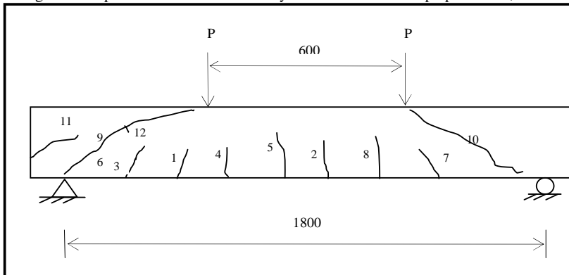
Fig. 9 Crack patterns of RC beam 20% rice husk ash contain 0.15% used engine oil, 20RHA/UEO
