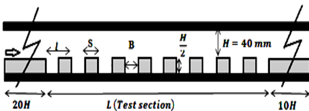
Fig. 1 Grooved channel
