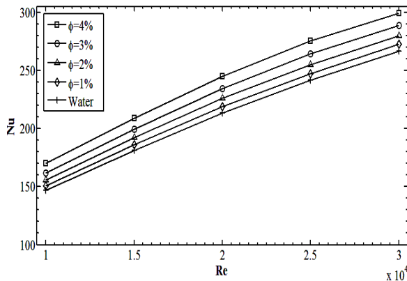
Fig. 6 Effect of volume fraction on Nusselt number of SiO 2 at different Reynolds number
