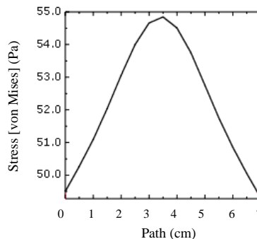
Fig. 9 Stress graph on the surface of kidney in a new model (a stone with a diameter of 1 cm and an embedding depth of 4 cm)
