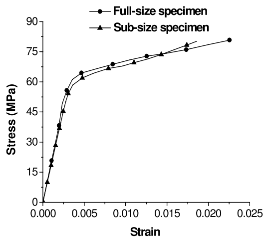
Fig. 4 Stress-strain behavior of sub-size and full-size tensile specimens for buffalo tibiae cortical bone
