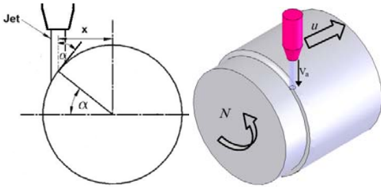
Fig. 1 Schematic diagram of AWJ turning
