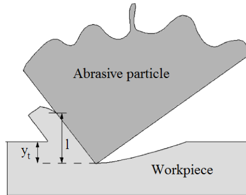
Fig. 2 Depth of cut and length of contact
