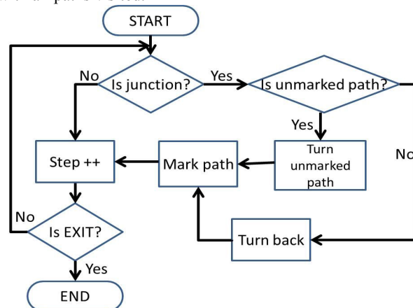
Fig. 2 Tremaux's algorithm [4]
