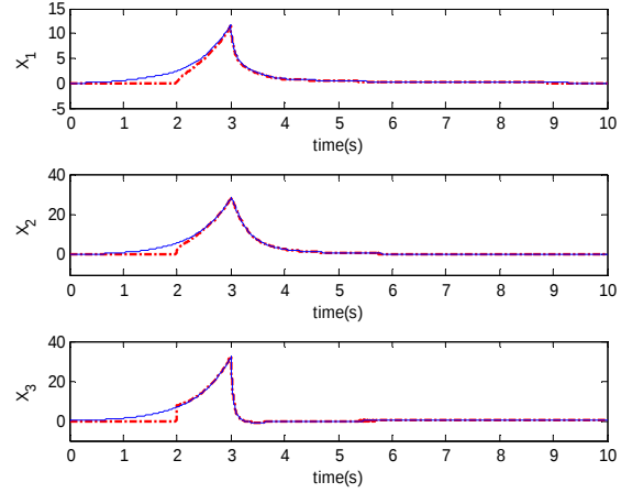
Fig. 1 Actual states (line), state estimations (dashed)
