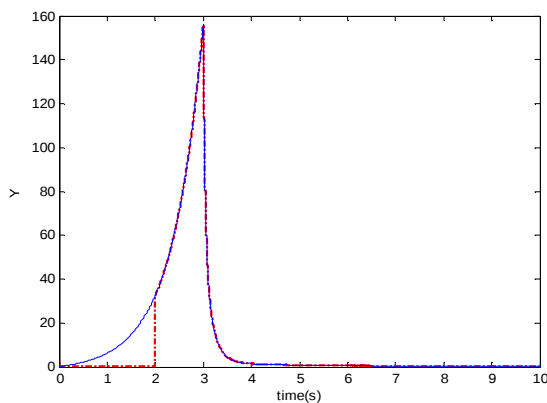
Fig. 3 Output signal of system (line) and observer's output (dashed).
