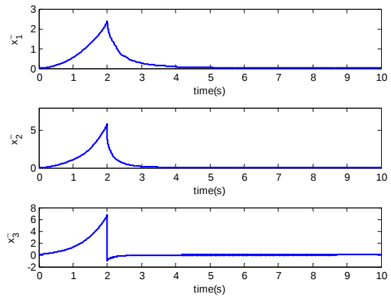
Fig. 2 Errors of state estimations using observer
