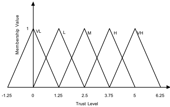
Fig. 1. Triangular Fuzzy Numbers Used in the model.
