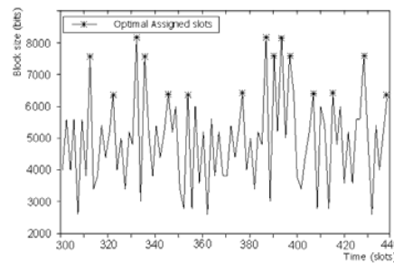
Fig. 5 (a) Assigned slots in OOS
