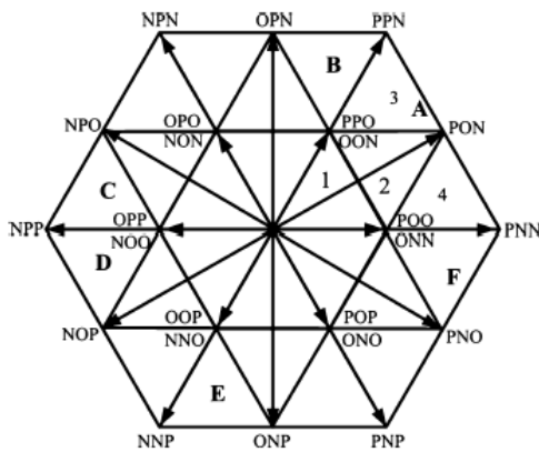
Fig. 2 Space vector diagram of a three-level inverter
