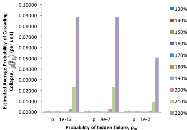
Fig. 1 Estimated average probability of cascading collapse \mu(\hat{P}_{C_i}) as a function of the hidden failure probability for IEEE-RTS96
