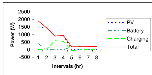
Fig. 5 The primary and secondary energy sources
