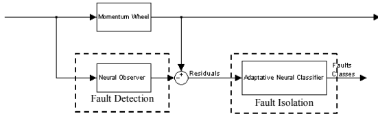
Fig. 1 General Structure of the neural network FDI Scheme
