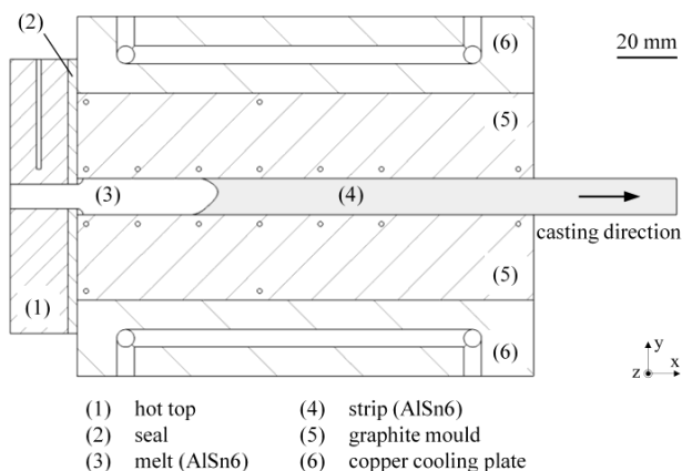
Fig. 1 Schematic of the casting mould to produce a single layer AlSn6 strip
