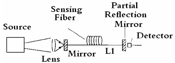
Fig. 7 Fabry-Perot interferometer-based fiber optic sensor
