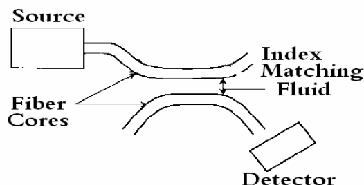
Fig. 4 Fiber Optic Sensor based on Evanescence
