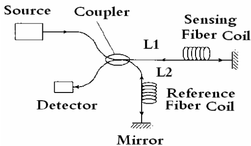
Fig. 6 Michelson interferometer-based fiber optic sensor
