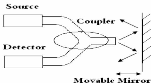
Fig. 3 Fiber Optic Sensor Using Reflection
