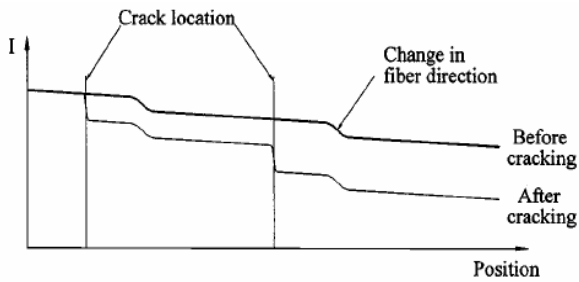
Fig. 13 Intensity along the fiber, measured by means of the optical time-domain reflectometry
