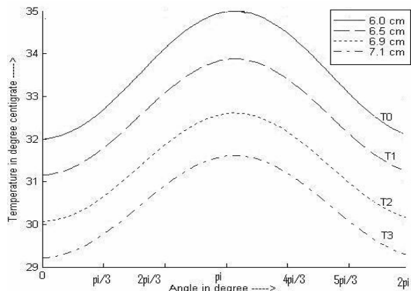
Fig. 4 Graph between Temperature T_i ( ^{\circ}C ) and angle v (deg.) for T_a=23^{\circ}C
