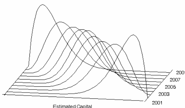
Fig. 4 Dynamic Modeling
