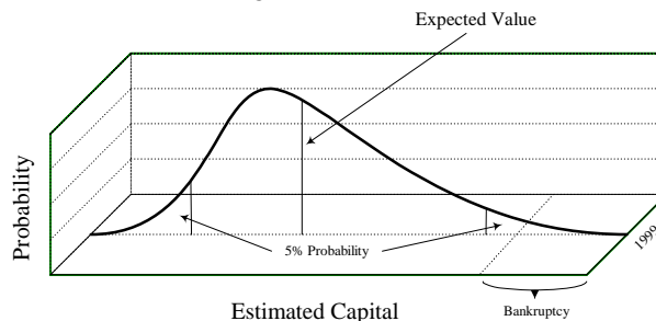
Fig. 3 Stochastic Modeling
