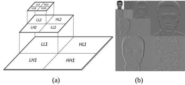
Fig. 2 Wavelet Transform (a) the pyramid scheme of resolutions; (b) an image transformed at level 3
