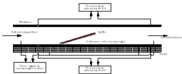
Fig. 1 Schematics of test apparatus
