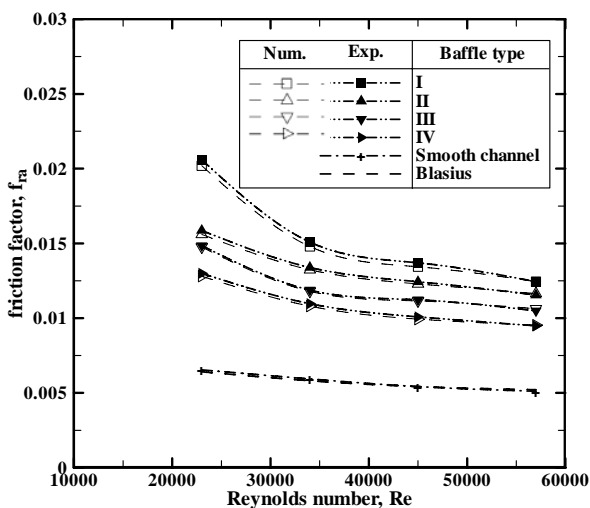
Fig. 9 Friction factor
